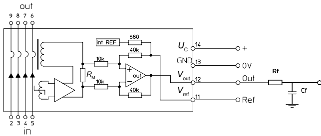
Figure 31: Test connection
