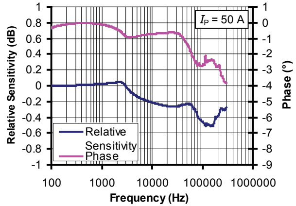
Figure 20: Frequency response
